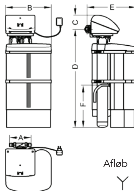
Figur 1: Installationsmål
